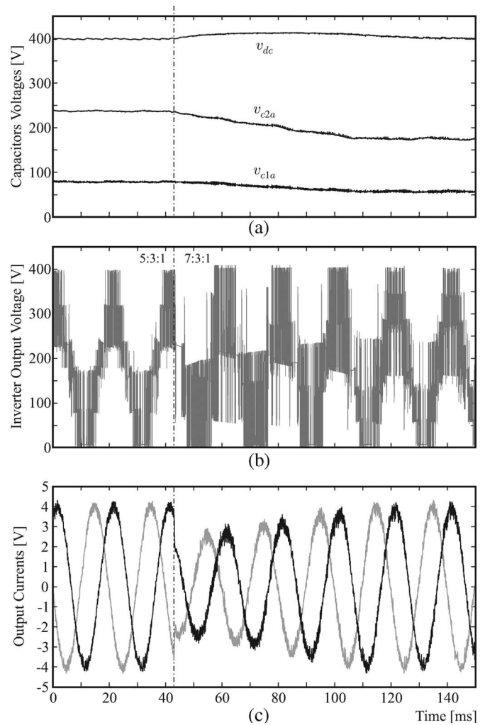
Fig. 11. Transition from 5 : 3 : 1 to 7 : 3 : 1 capacitor voltage ratio. (a) Capacitor voltages. (b) Output voltage. (c) Output currents.
